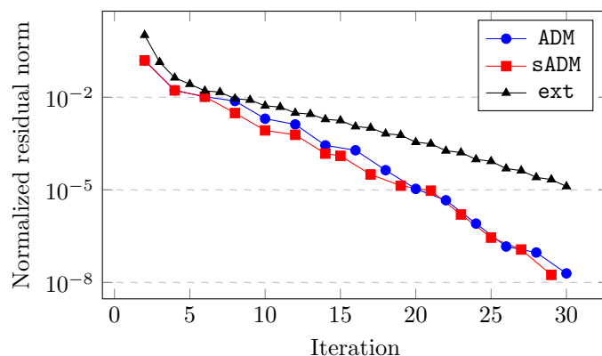
FIG. 2. Behavior of the residual produced by solving the convection-diffusion equation with block rational Krylov methods with different choices of poles. Note: color appears only in the online article.
